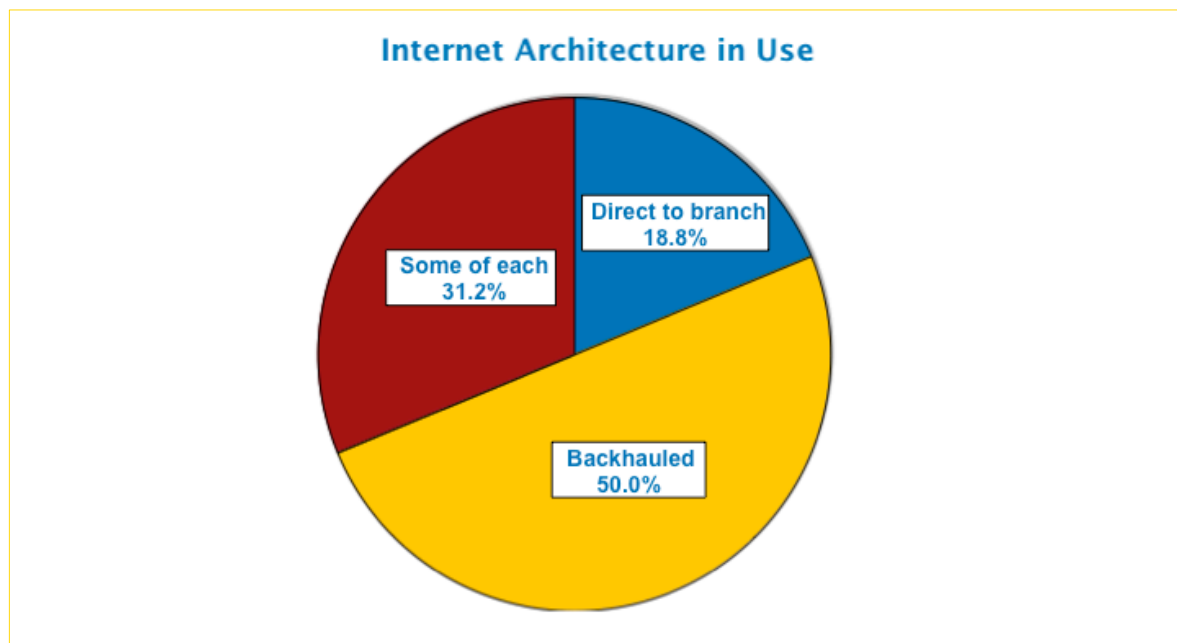
Figure 2: Direct-to-Branch Internet
